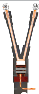
Series Heat Shrinkable Terminations Suitable for PVC/XLPE Cables upto 3.3kV.
